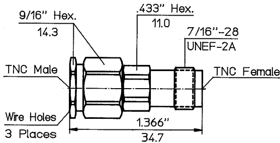
TNC-Interfaces as per MIL-C-87104/2
