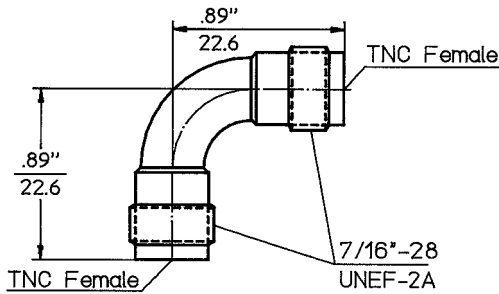
TNC-Interfaces as per MIL-C-87104/2
