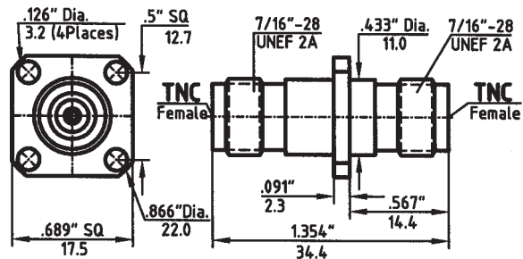
TNC-Interfaces as per MIL-C-87104/2
