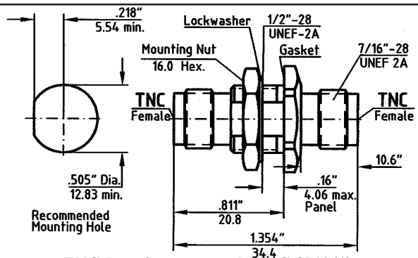
TNC-Interfaces as per MIL-C-87104/2
