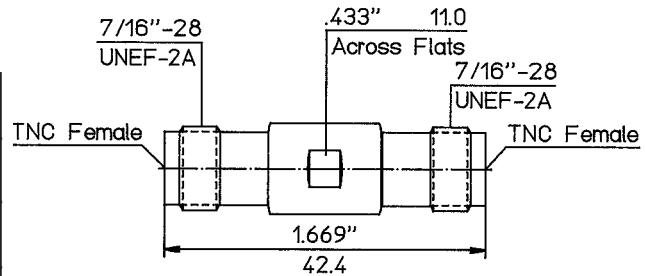
TNC-Interfaces as per MIL-C-87104/2
