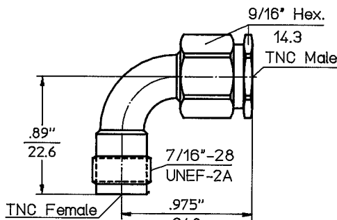
TNC-Interfaces as per MIL-C-87104/2
